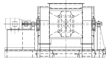
Arrangement 7 Direct Drive DIDW c/w inlet boxes
