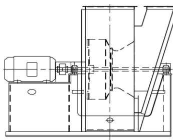
Arrangement 7 Direct Drive SISW c/w inlet box
