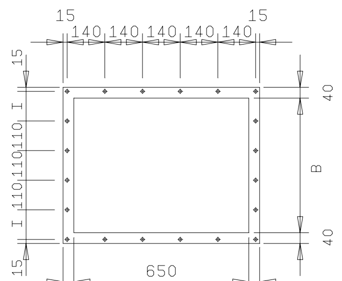
DISCHARGE FLANGE DETAIL 20 HOLES Ø 12mm
